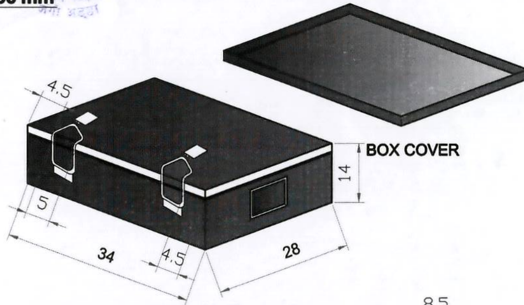
ISOMETRIC VIEW ASSEMBLY
